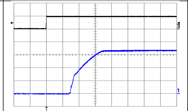
Figure 17. Turn-on transient at full rated load current (resistive) plus 10,000 F at V_{in} = 24\text{ V} , triggered via ON/OFF pin. Top trace: ON/OFF signal (5 V/div.). Bottom trace: output voltage (1 V/div.) Time scale: 1 ms/div.
