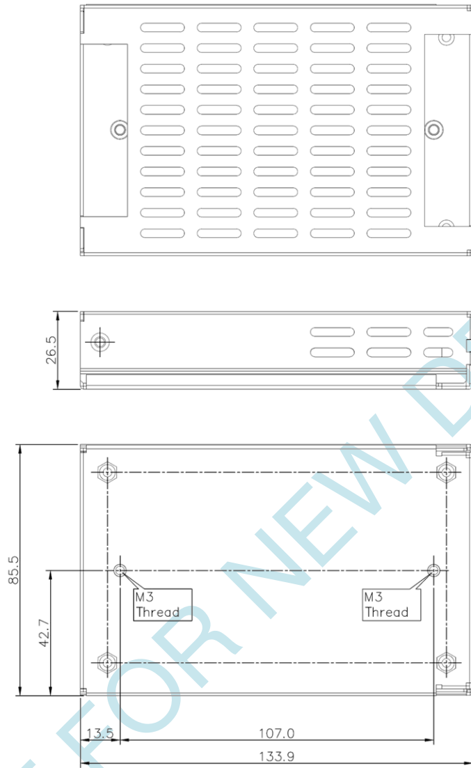
MECHANICAL OUTLINE DIMENSIONS ALL DIMENSIONS ARE IN MM. GEN. TOLERANCE: ±1.0 mm
