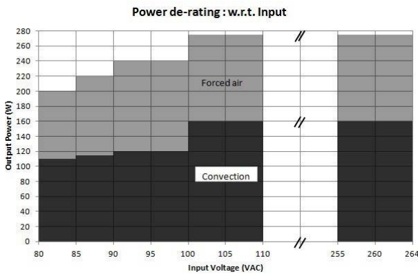
Figure1. Derating Curves
